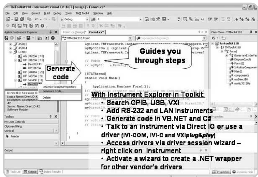
Figure 12. Toolkit saves time. It searches for instruments, writes to them regardless of I/O type, shows all choices for the next function call, writes the VB .NET or C# commands for that function, and gives you context-sensitive help—all in one environment.
