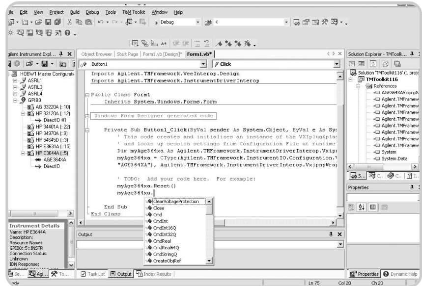
Figure 6. Agilent's T&M Programmers Toolkit using a VXiPlug&play WIN32 power supply driver in VB .NET after being wrapped by the Driver Wizard.
