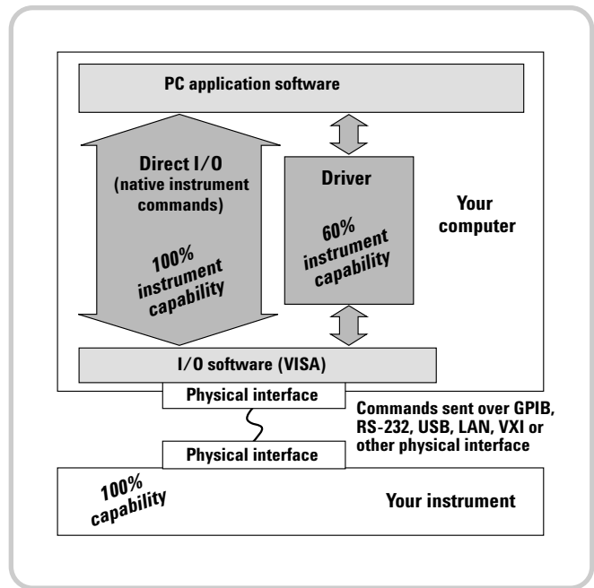
Figure 9. If you are using a driver and need to access instrument functions the driver doesn’t have, you can send direct SCPI or ASCII commands, or go through the driver with pass-through commands to control the instrument directly. This gives you the convenience of drivers, with the 100% coverage of direct I/O.
