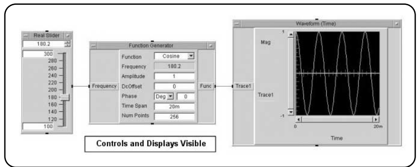
Figure 7. A typical VEE panel driver. VEE is the fastest T&M graphical language to learn. Fill in the boxes, and the VEE panel driver generates code for you. See http://we.home.agilent.com/upload/cm_upload/tmo/downloads/E206HPVEE_TESTENGR_EVAL.pdf
